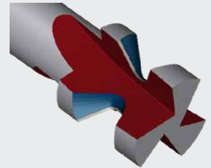
Radial Form Cutters
